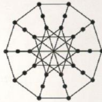
Levi graph
