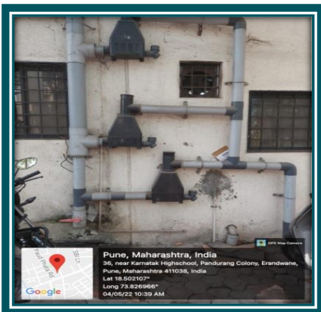
Rain Water Harvesting System, Bore Well and Recharge Well
